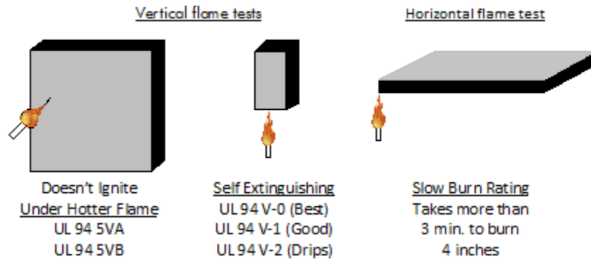
Figure 3: UL Burn Test Images
